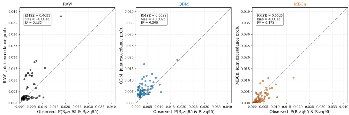
Figure 5. Pairwise probability that both gauges exceed their 95th wet-day percentile on the same day, shown as the seven-model mean against observations. MBCn lies closest to the 1:1 line and is the only method without a systematic tilt.
