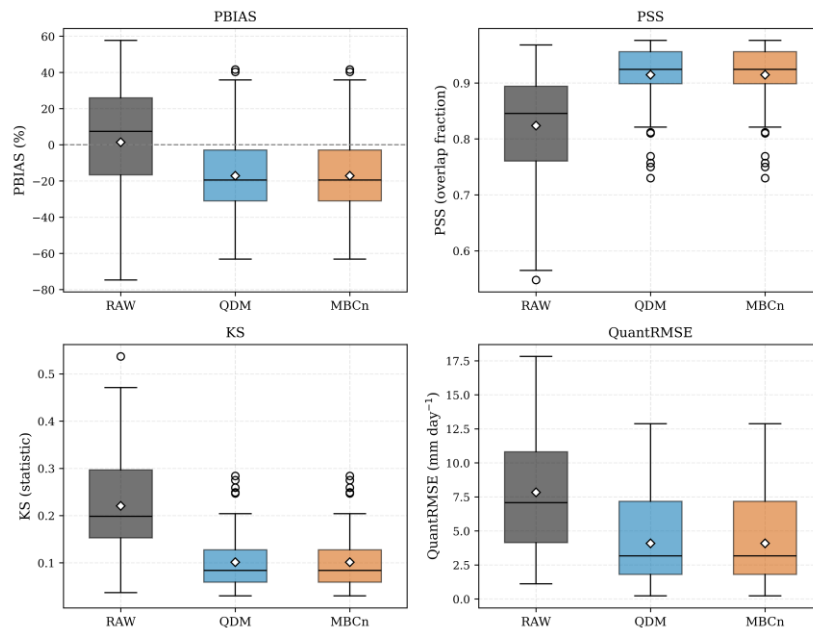
Figure 3. Single-site skill for RAW, QDM, and MBCn over the withheld validation period, one point per gauge-model pair (n = 84). Diamonds mark the mean. The QDM and MBCn distributions coincide exactly, by construction.
