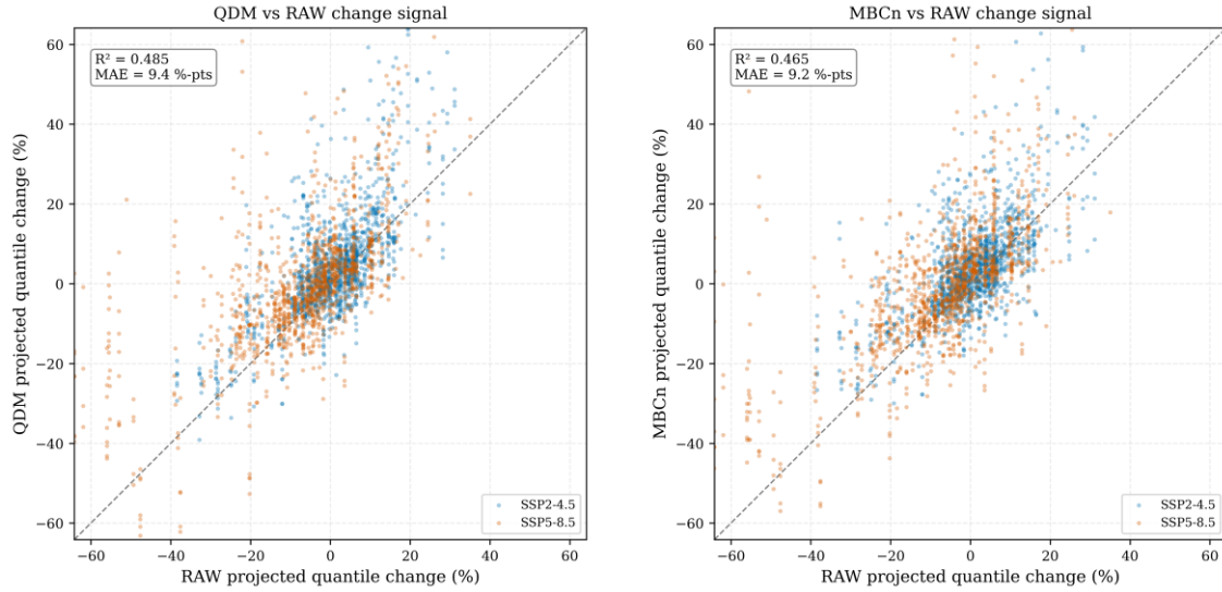
Figure 6. Raw versus corrected projected change in wet-day quantiles for every gauge, model, pathway, and future period. QDM and MBCn preserve the model-projected quantile-change signal to a similar degree.
